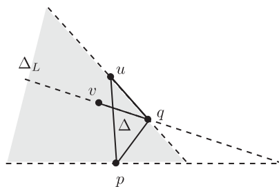
Fig. 18. E(p) does not contain a cycle.
