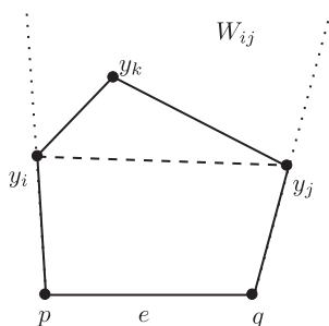
Fig. 11. An empty convex pentagon yields an empty convex quadrilateral py_iy_jq , with y_i, y_j non-consecutive.
