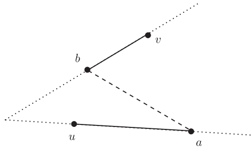
Fig. 4. A T_2 -configuration and the charged diagonal ab .
