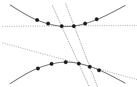
Fig. 9. Lower bounds for T_2 and T_2^* .
