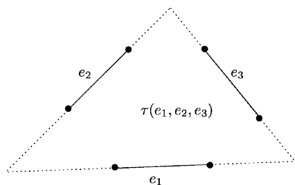
Fig. 2. A T_3 -configuration.
