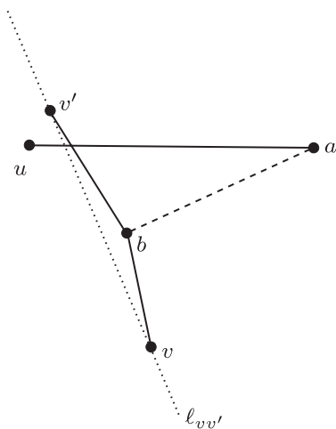
Fig. 7. Showing that \ell_{vv'} must separate a and b .
