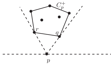
Fig. 15. A point p counted in H' .
