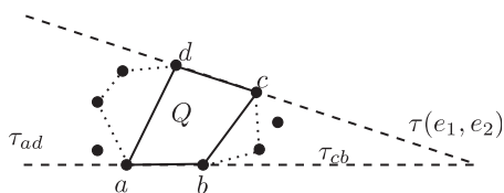
Fig. 13. The structure in the proof of Lemma 5.5.
