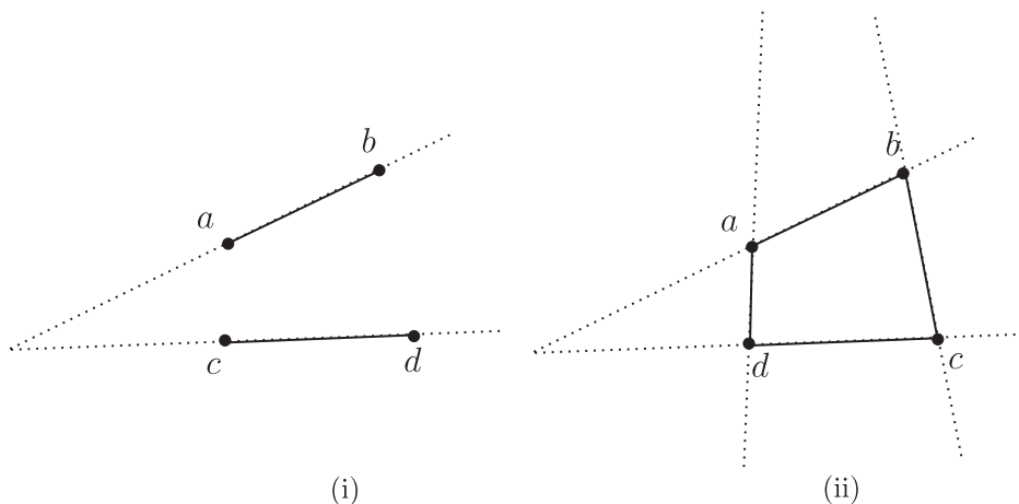
Fig. 1. (i) A pair of edges (ab, cd) that is counted in T_2 : They lie in convex position and define an empty wedge. (ii) A quadrilateral abcd that is counted in T_2^* : Both wedges are empty.
