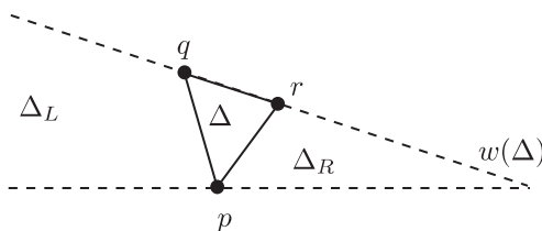
Fig. 17. An empty triangle \Delta and the partition of its associated wedge.
