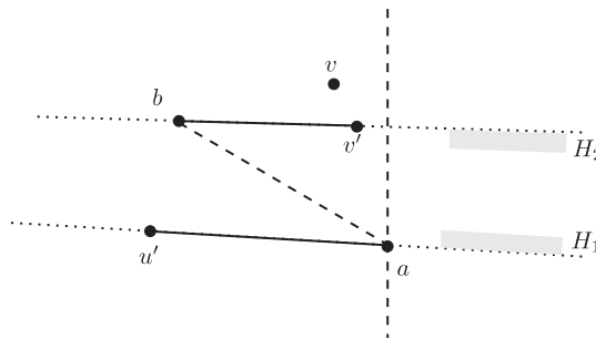
Fig. 5. v has to lie in H_1 .
