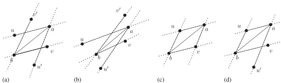
Fig. 6. The various cases in the refined analysis of T_2 .
