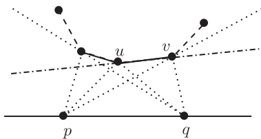
Fig. 19. Pointed triangles with edge pq that cannot be extended to an empty convex pentagon.
